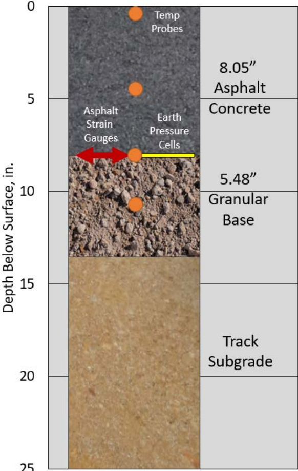
FIGURE 1 Thick-lift cross section (S9).
