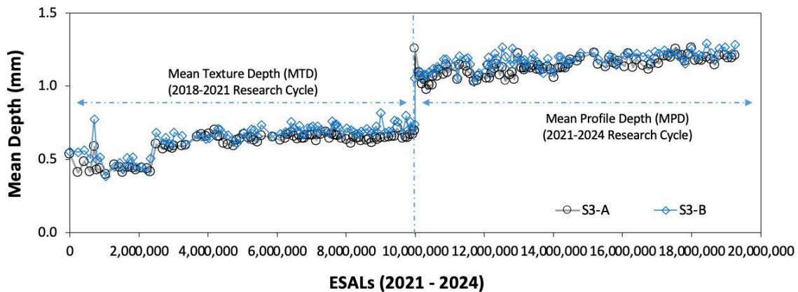
FIGURE 22 Surface macrotexture measurements.
