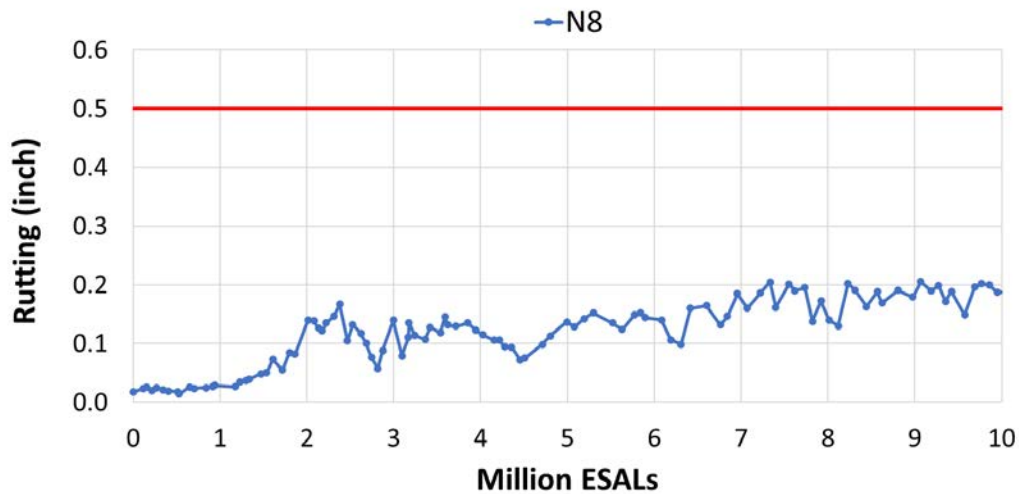
FIGURE 12 Field rutting data of Section N8.
