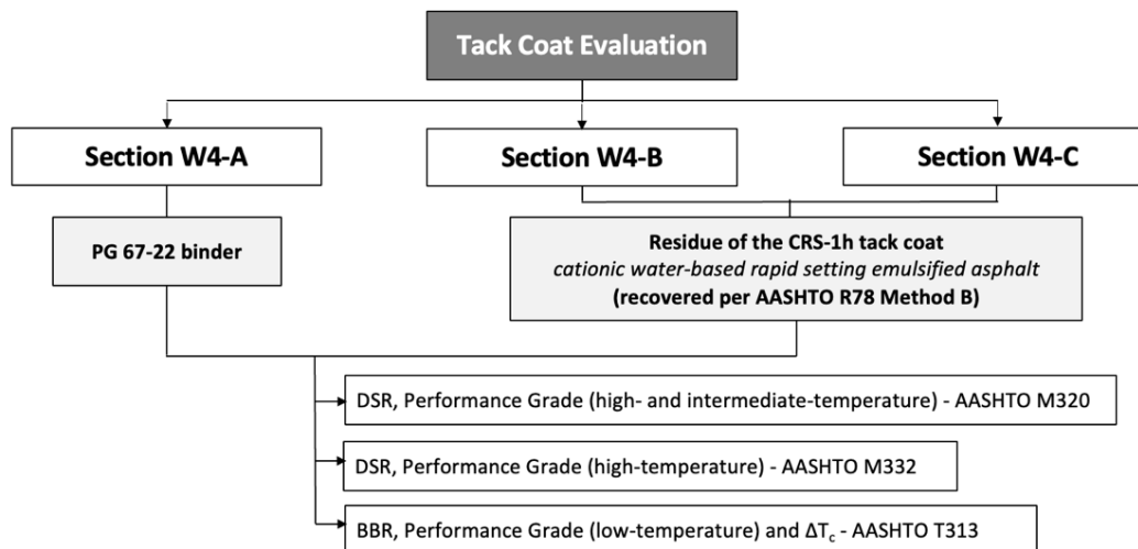
FIGURE 5 Binder testing matrix.
