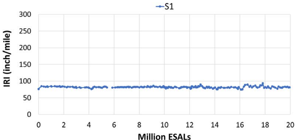
FIGURE 9 Field smoothness data of Section S1.
