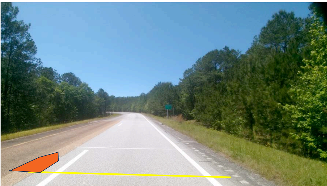
FIGURE 18 Subsection N13-B OGI, 0.19-inch rutting, 0.8% cracking (April 2024).
