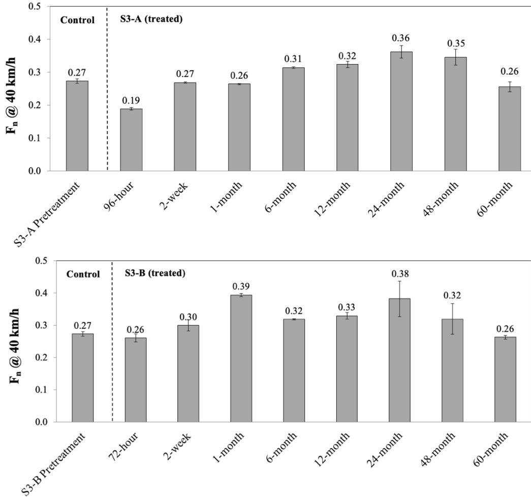
FIGURE 18 Average F_n at 40 km/h at several time intervals.
