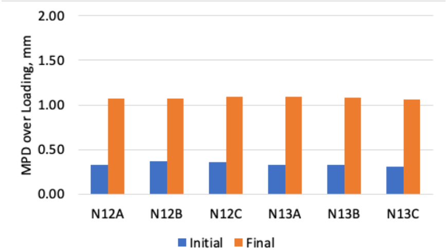
FIGURE 9 Mean texture depth comparison of N12 and N13.
