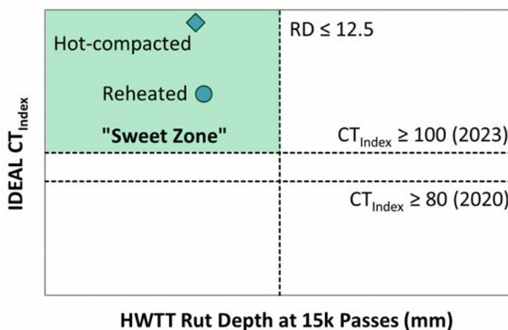
FIGURE 10 HWTT-versus-IDEAL-CT performance diagram of N8 surface mix.
