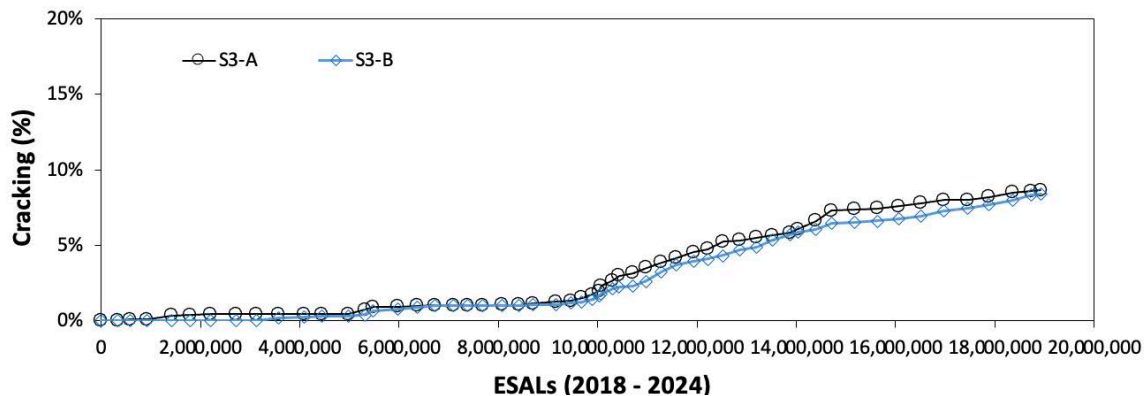
FIGURE 20 Field cracking measurements.
