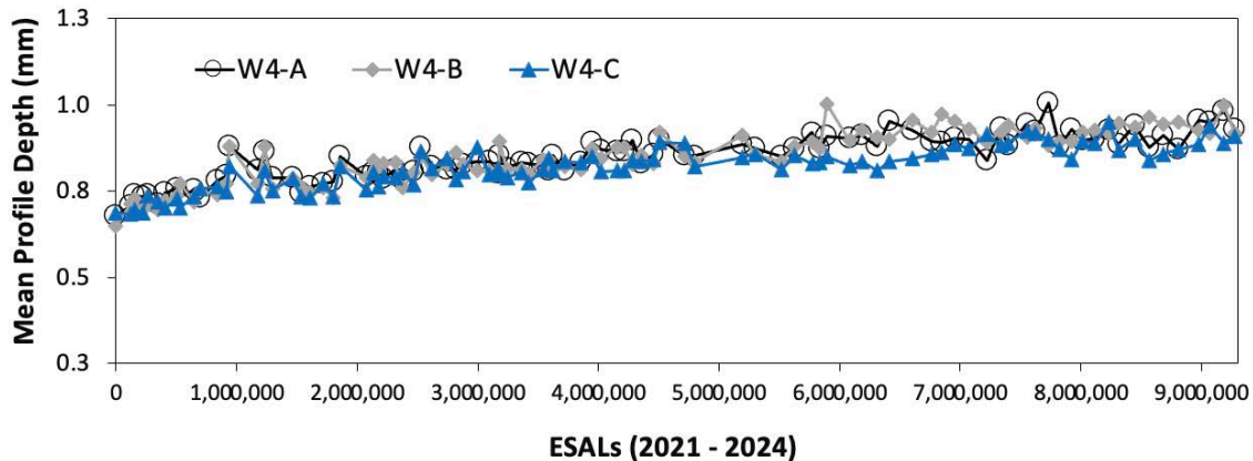
FIGURE 14 Surface macrotexture (MTD) measurements.
