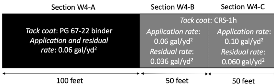
FIGURE 4 Test track Section W4 layout.
