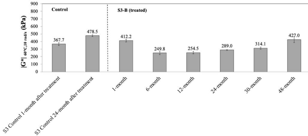
(b) S3 control vs. S3-B FIGURE 9 Effect of field aging on |G^*| at 60°C and 10 rad/s.
