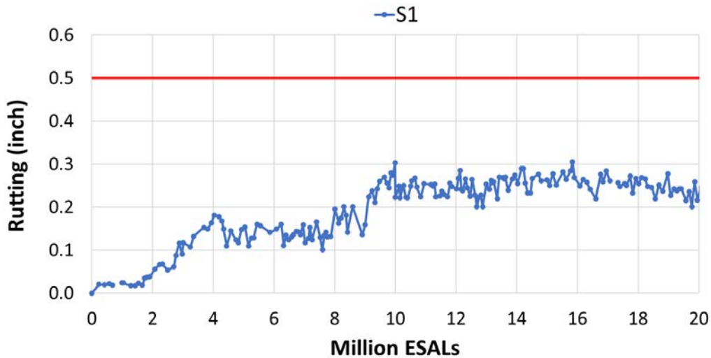
FIGURE 8 Field rutting data of Section S1.
