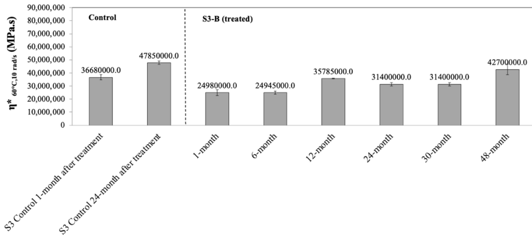
(b) S3 control vs. S3-B FIGURE 10 Effect of field aging on \eta^* at 60°C and 10 rad/s.
