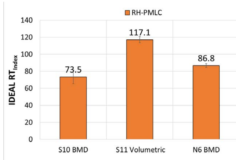
FIGURE 10 IDEAL RT_{Index} results of reheated PMLC specimens.
