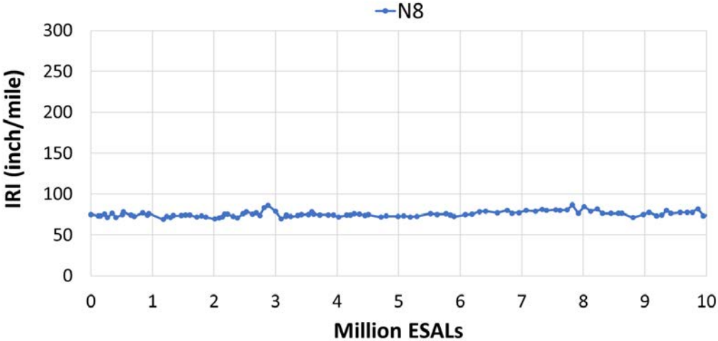
FIGURE 13 Field smoothness data of Section N8.
