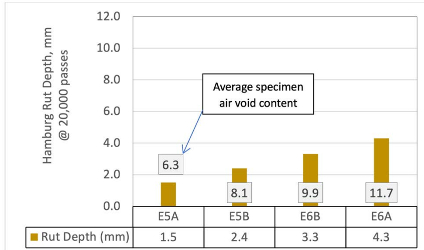
FIGURE 15 Hamburg test results of subsections E5A, E5B, E6A, and E6B.
