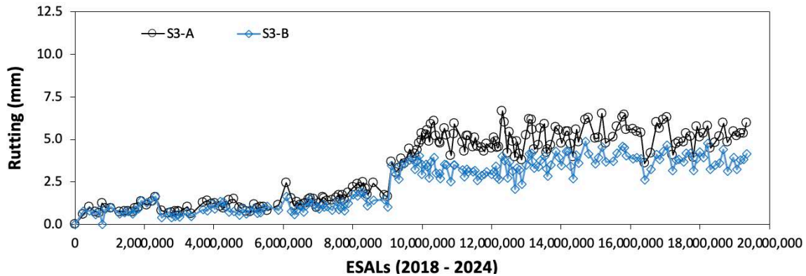
FIGURE 19 Field rut depth measurements.
