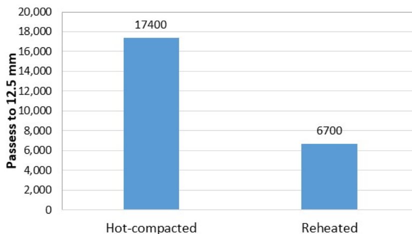
FIGURE 18 HWTT results of N9 surface mix.
