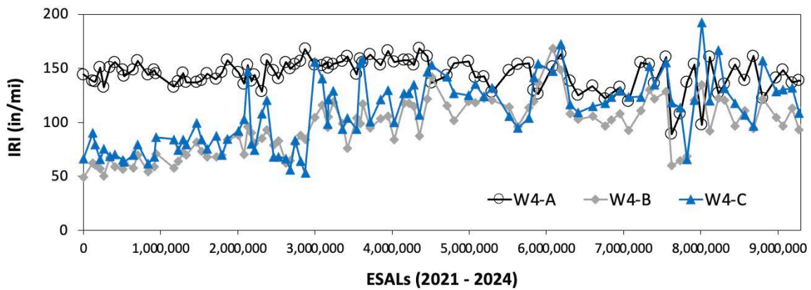
FIGURE 13 Ride quality (IRI) measurements.
