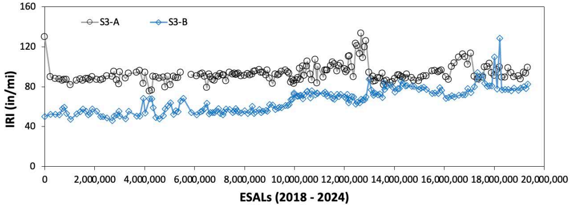
FIGURE 21 Ride quality (IRI) measurements.
