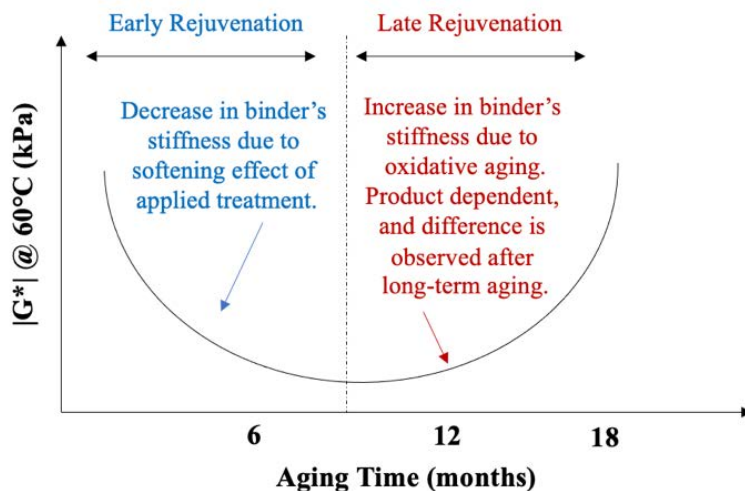
FIGURE 11 Hypothesized behavior of spray-on rejuvenator products.
