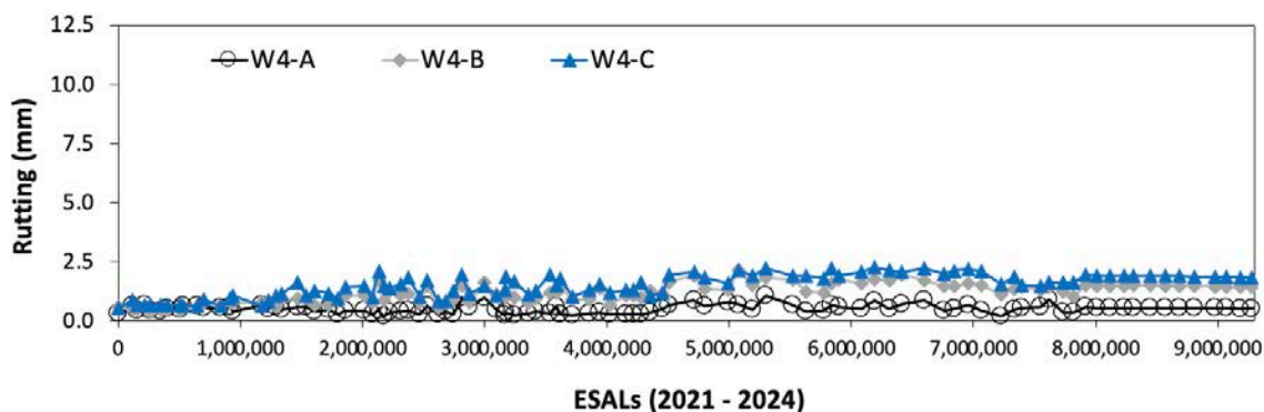
FIGURE 11 Field rut depth measurements.
