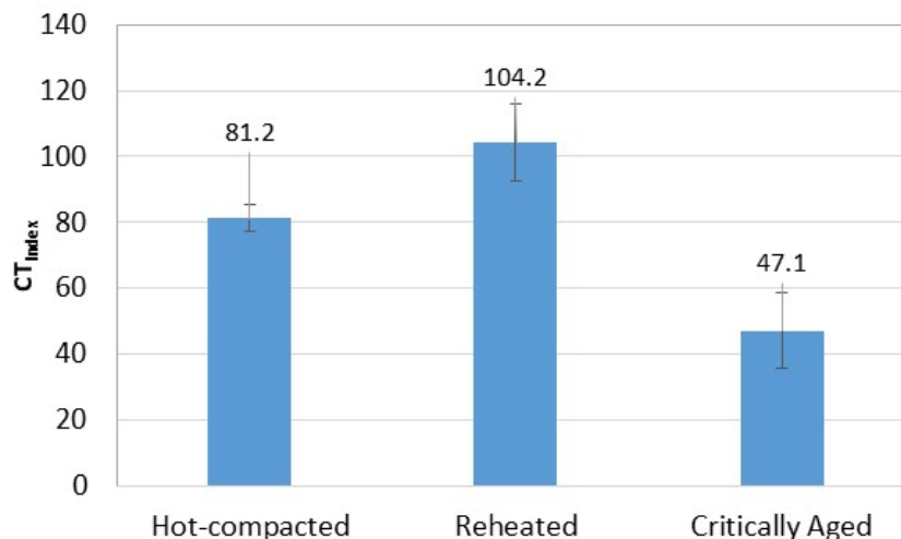
FIGURE 17 IDEAL-CT results of N9 surface mix.
