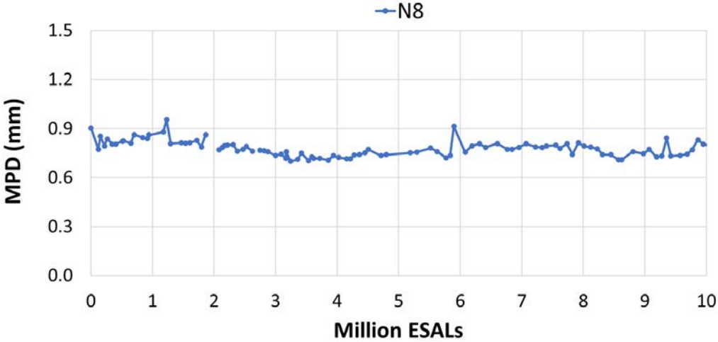
FIGURE 14 Field surface texture data of Section N8.
