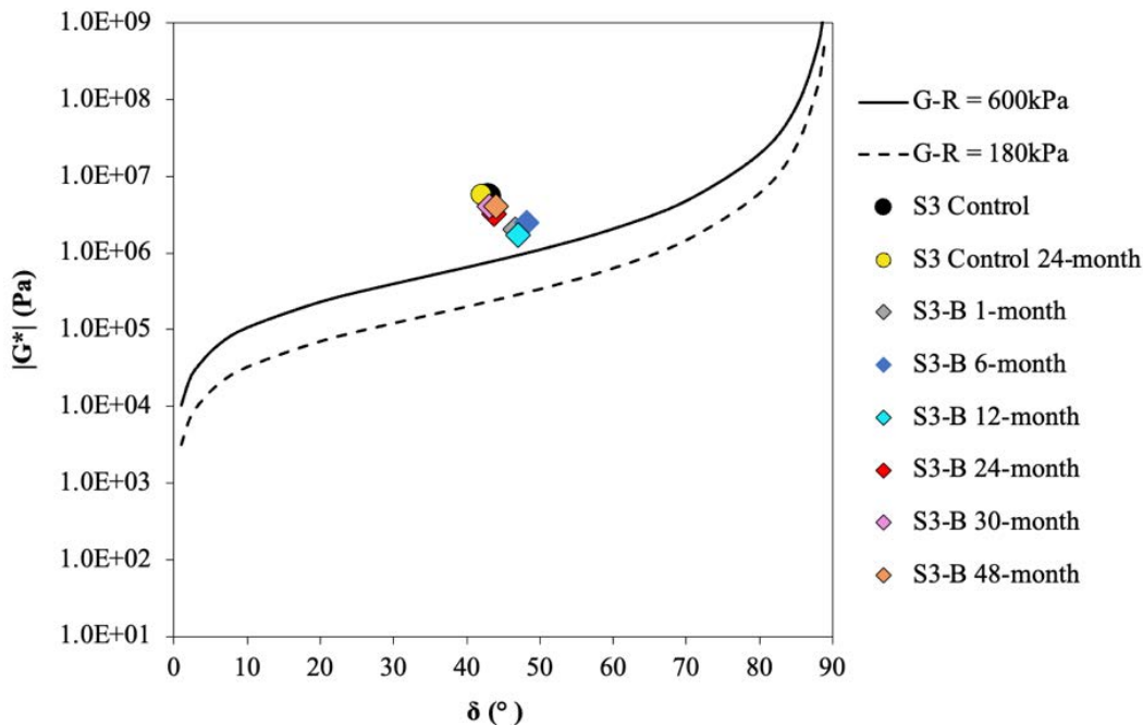
(b) S3 control vs. S3-B
