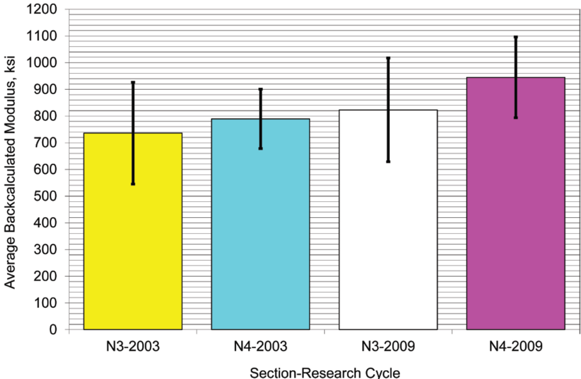
Figure 3.47 Temperature-Normalized Backcalculated Moduli
