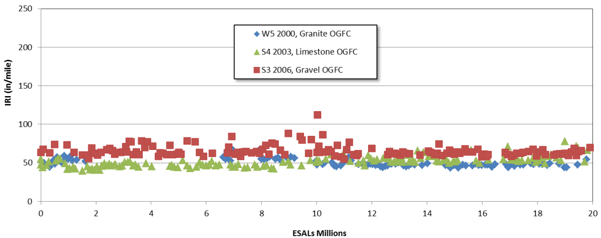
Figure 2.8 IRI for OGFC Test Sections Through Two Cycles
