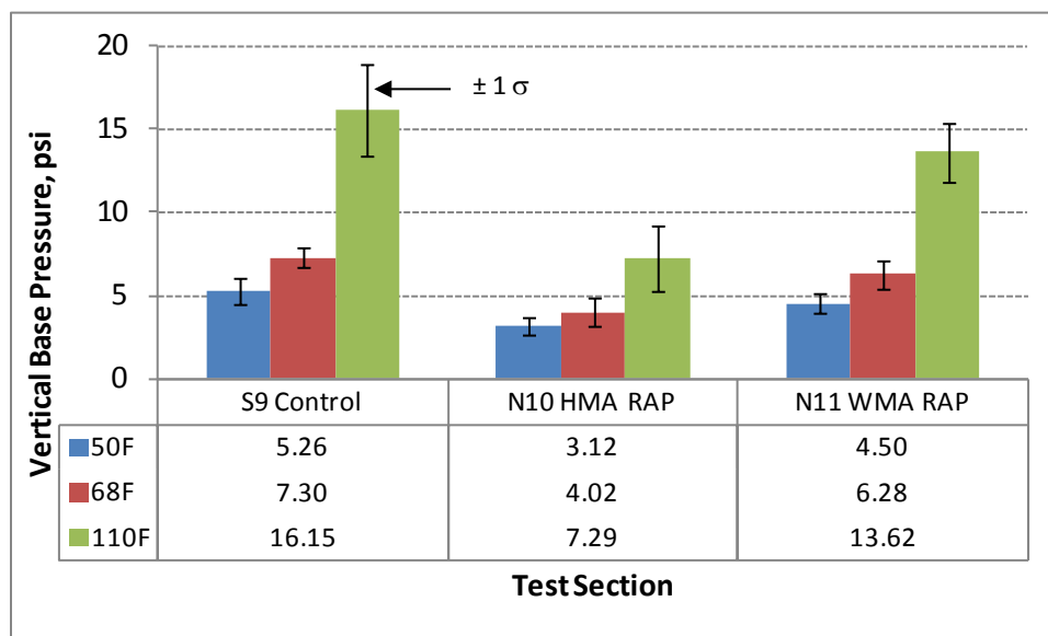
Figure 3.11 Average Vertical Pressure at Reference Temperature
