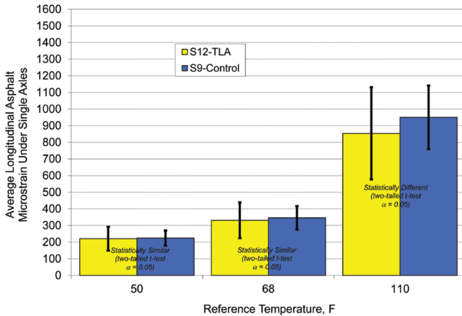
Figure 3.64 Temperature-normalized Asphalt Strain
